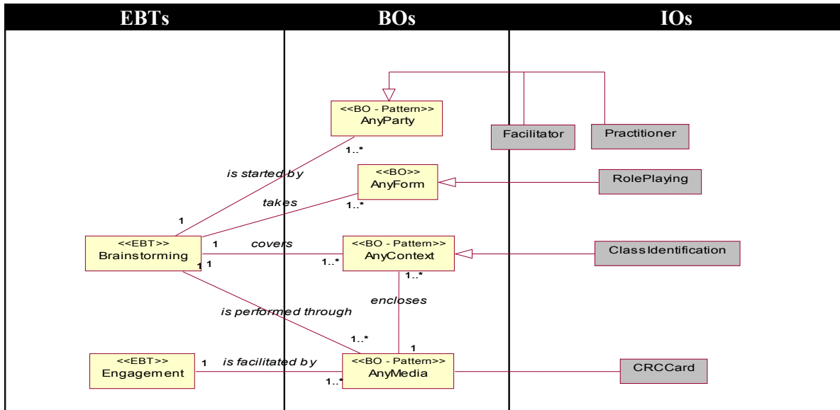
Figure 4: Brainstorming Analysis Pattern, stable object model Applicability
