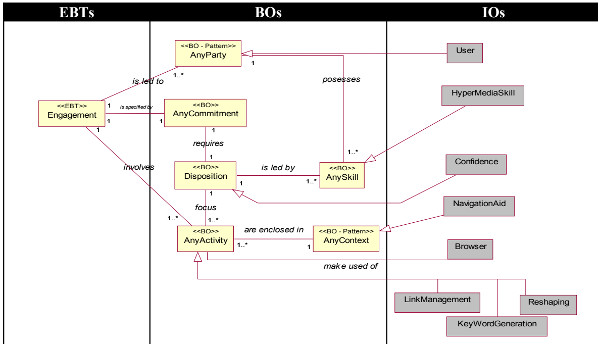
Figure 6: Stable Conceptual Map Creation
