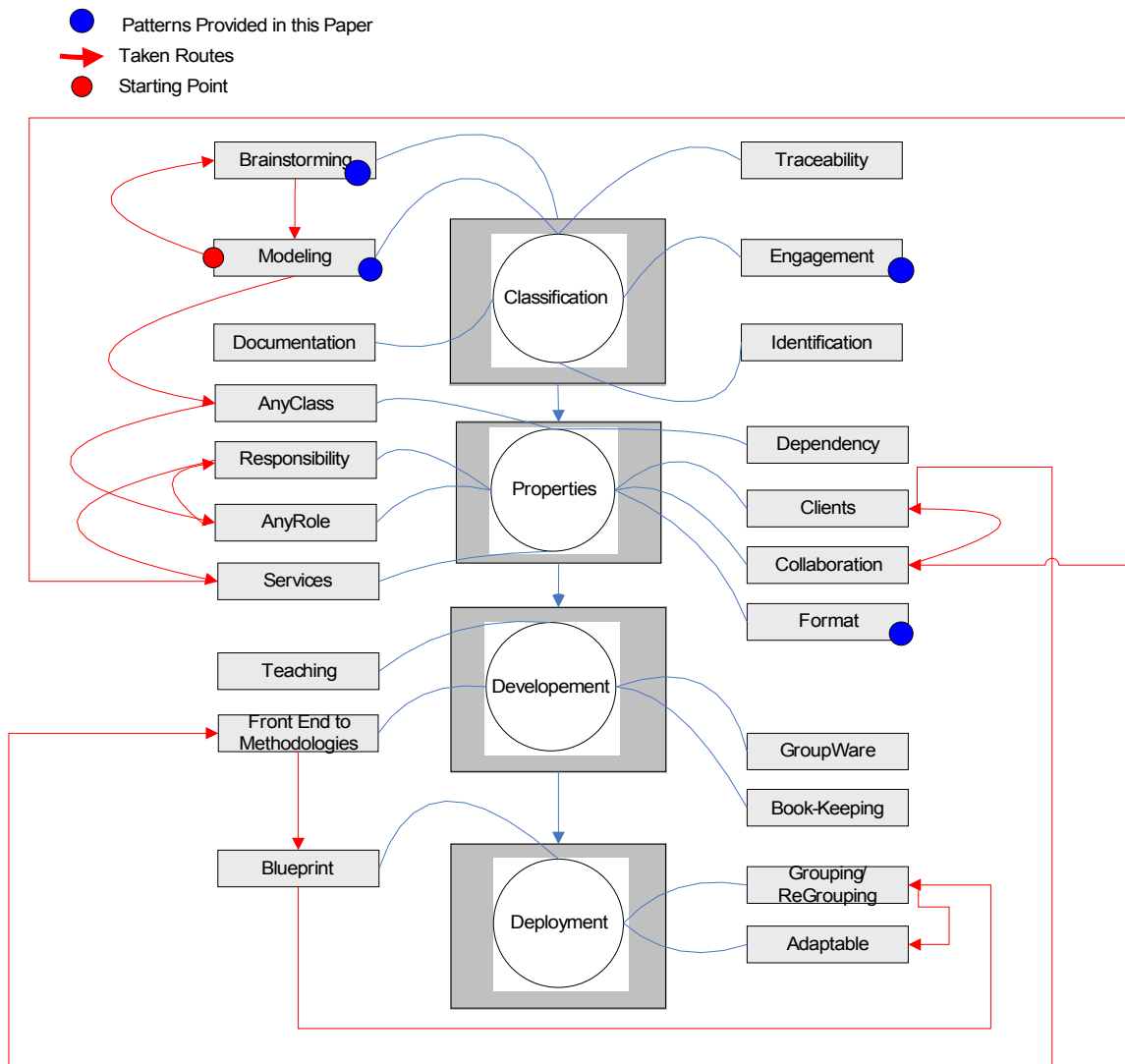
Figure 2: A Pattern language for CRC Cards – Achieving the Modeling Goal.
