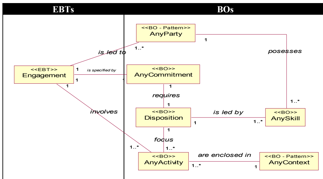
Figure 5: Engagement Analysis Pattern stable object model
