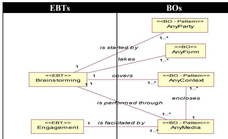
Figure 3: Brainstorming Analysis Pattern stable object model.
