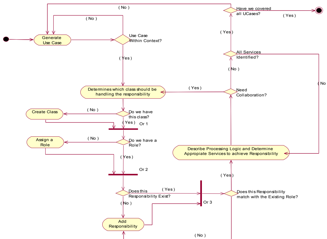
Figure 7: CRC Modeling Accuracy Test Process Flow
